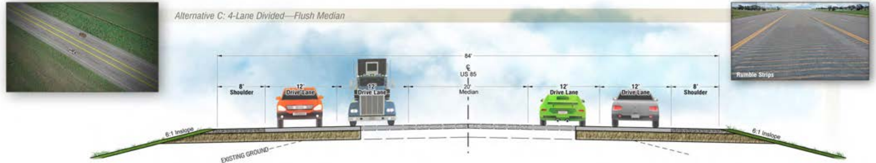
Figure 16, Typical Section for Divided, Flush Median
