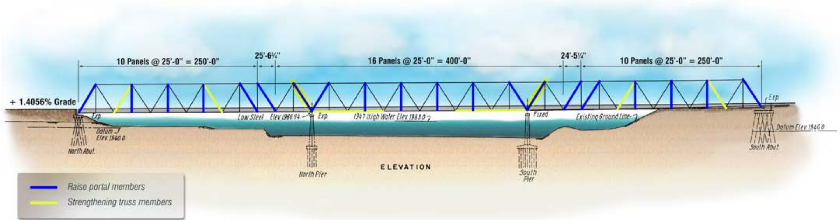
Figure 80, Option LX-1: Scope of Rehabilitation
