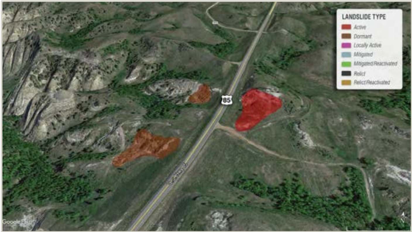
Figure 54, Google Earth Aerial Image of Mapped Landslides (Southern Portion of Badlands)
